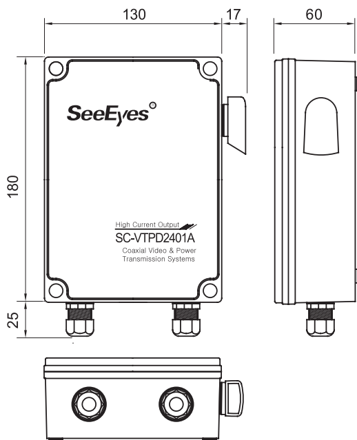
送信機(SC-VTPD2401A/D)
